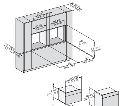
H 6x80BP, H 6x70 BM, ESW 6x85, H 6x80-2BP, H7xxx BM/BP/BPX, BMX, ESW7x70, EVS7670, Installation drawing, Flush inset, NA
